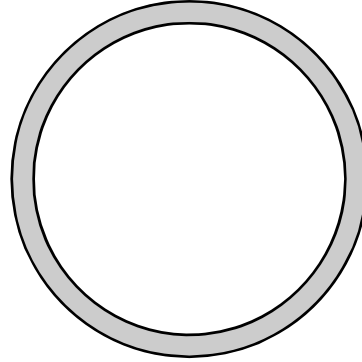
1 3/4" #92900 Outside: 1.865" Inside: 1.635"
