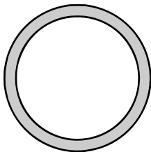
1" #92400 Outside: 1.100" Inside: .932"
