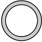
5/8" #92100 Outside: .740" Inside: .596"
