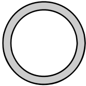
3/4" #92200 Outside: .875" Inside: .707"
