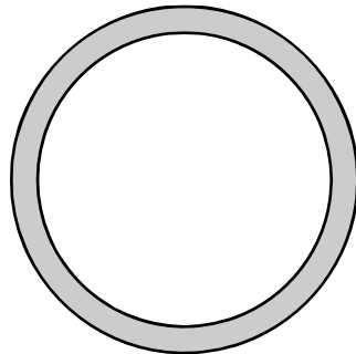
1 1/2" #92800 Outside: 1.640" Inside: 1.396"
