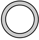
1/2" #92000 Outside: .670" Inside: .526"
