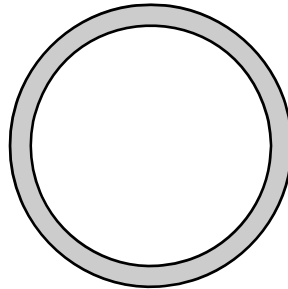
1 3/8" #92700 Outside: 1.480" Inside: 1.264"
