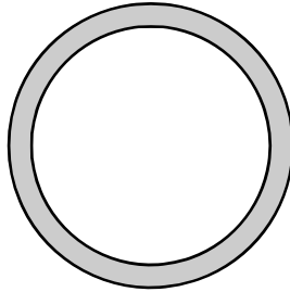
1 1/4" #92600 Outside: 1.375" Inside: 1.159"
