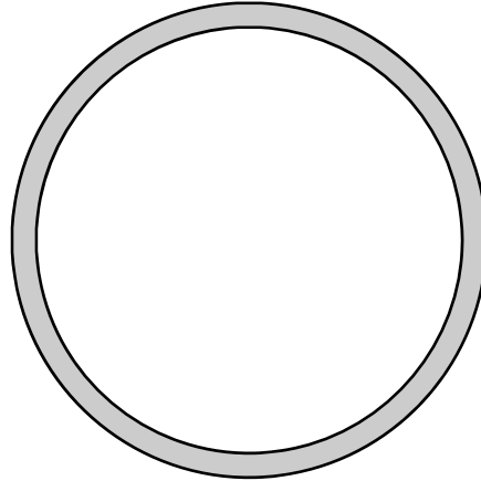
2" #92950 Outside: 2.240" Inside: 2.016"
